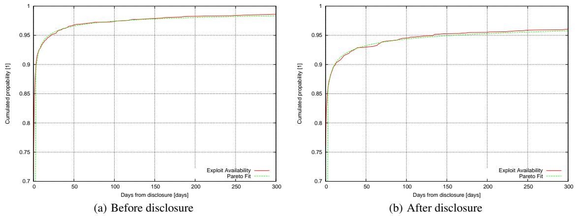
Figure 7: Overall exploit availability matches a Pareto distribution. \alpha decreases from 0.43 to 0.27 after disclosure reflecting a slowdown of the availability rate around disclosure.
