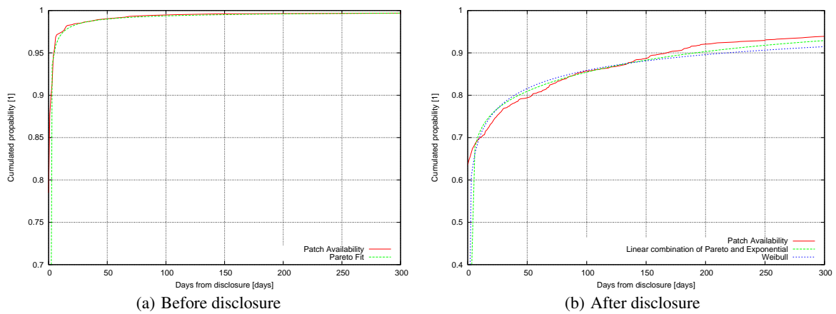
Figure 8: Overall patch availability before disclosure matches a Pareto distribution. \alpha = 0.62 reflects a higher rate in patch availability than in exploit availability right before disclosure. After disclosure a Weibull distribution is a reasonable match to the patch availability. A good match is obtained with a linear combination of a Pareto and an Exponential distribution.
