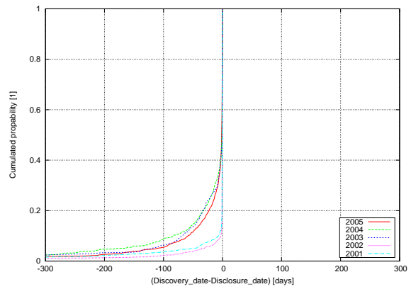
(b) CDF of discovery- vs. disclosure-date
